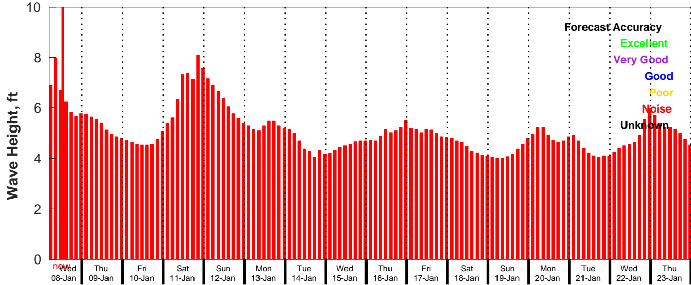
GFS Wave Forecast for NDBC 46069 from 08-Jan-2025 04:00:00 to 24-Jan-2025 04:00:00
