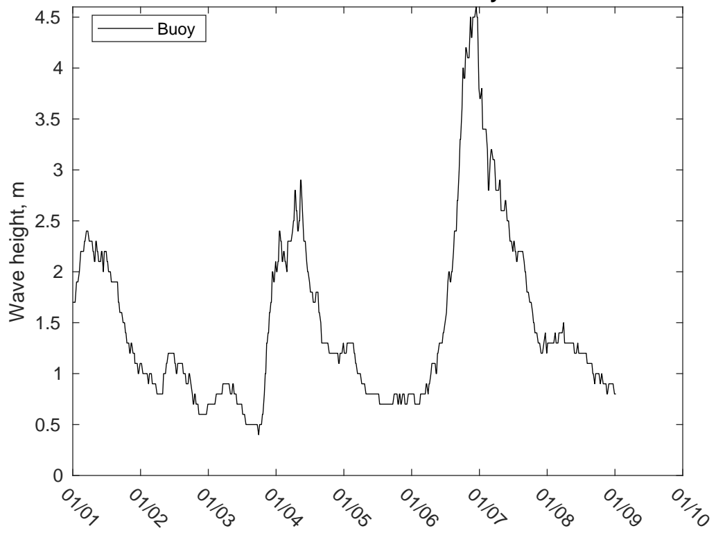
NDBC 41013 vs CMEMSWaves: 10 to 16 day forecast
