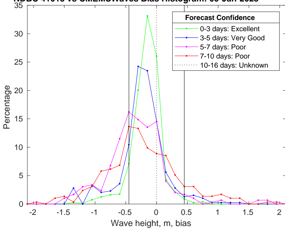
NDBC 41013 vs CMEMSWaves Bias Histogram: 09-Jan-2025
