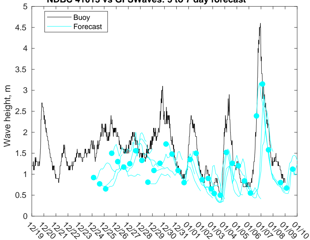
NDBC 41013 vs GFSWaves: 5 to 7 day forecast
