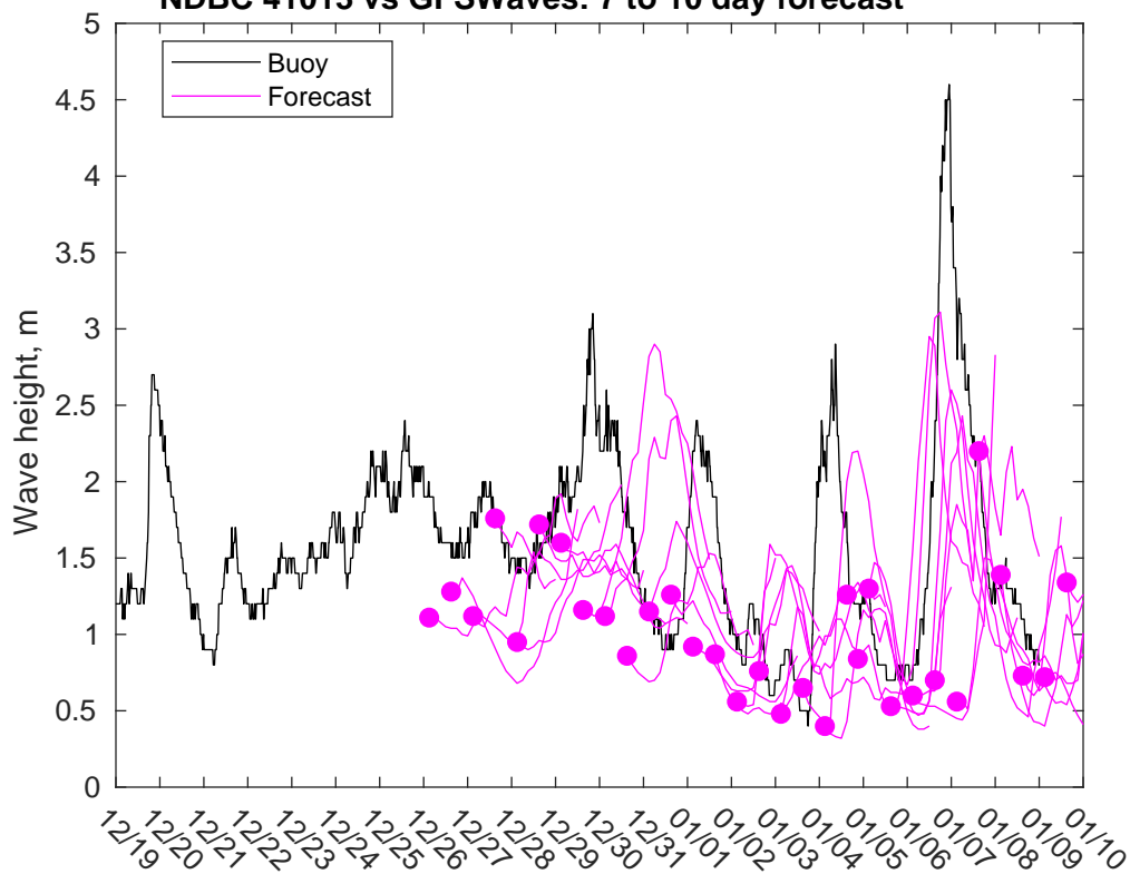
NDBC 41013 vs GFSWaves: 7 to 10 day forecast
