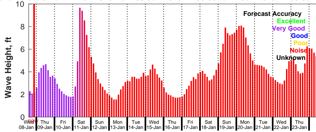
GFS Wave Forecast for NDBC 41013 from 08-Jan-2025 14:00:00 to 24-Jan-2025 14:00:00
