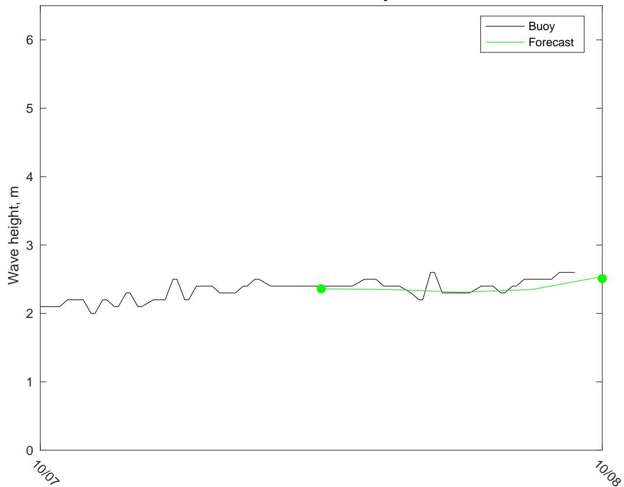
NDBC 42002 vs GFSWaves: 0 to 3 day forecast
