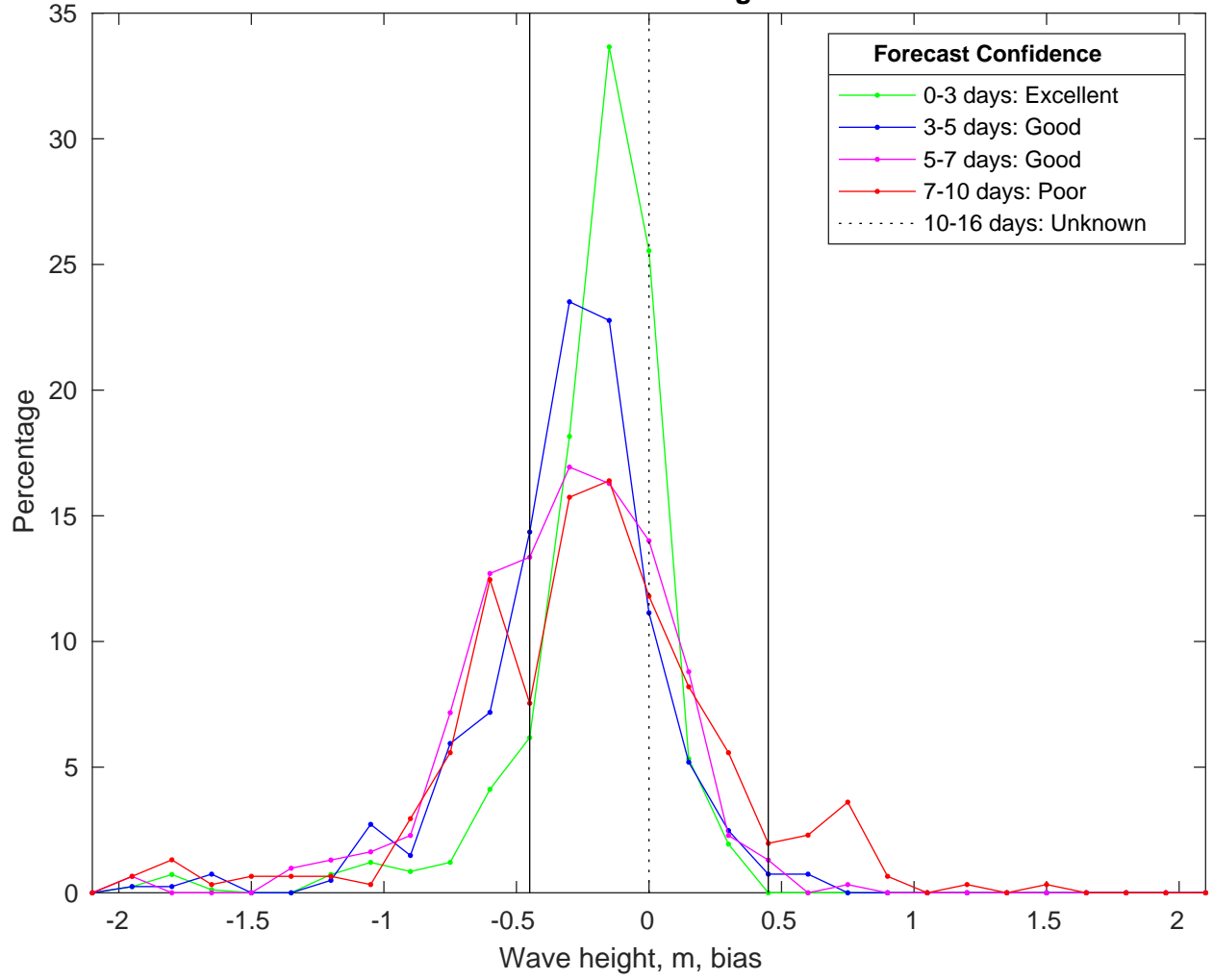
NDBC 42020 vs CMEMSWaves Bias Histogram: 09-Jan-2025
