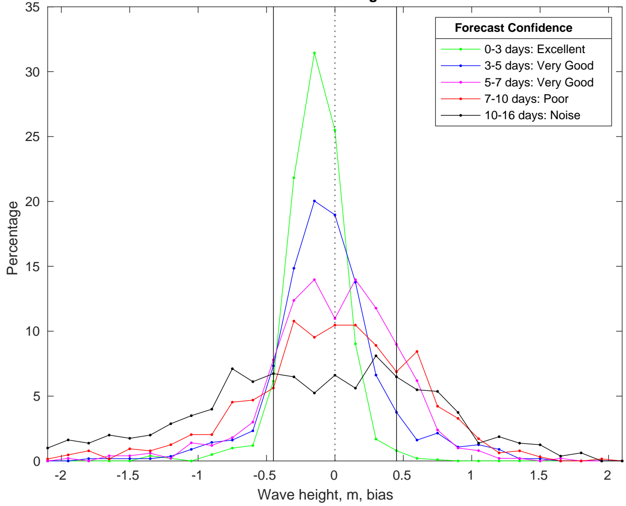
NDBC 42020 vs GFSWaves Bias Histogram: 09-Jan-2025
