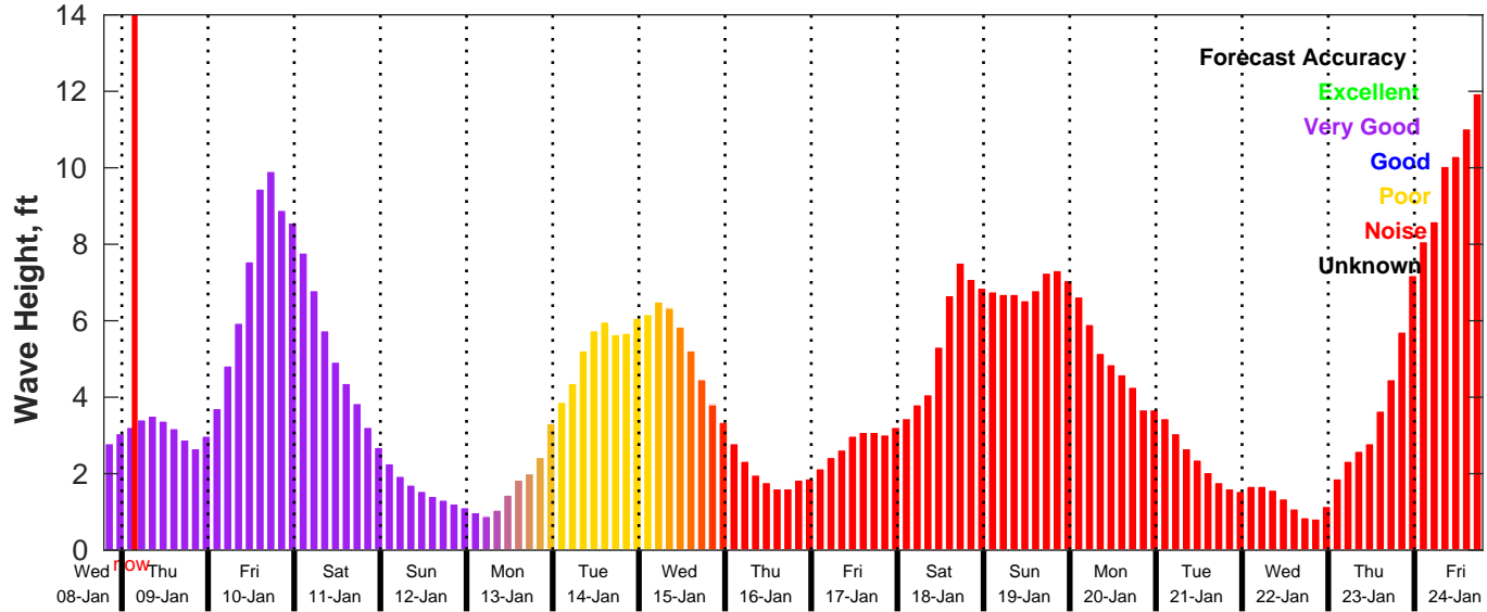
GFS Wave Forecast for NDBC 42040 from 08-Jan-2025 19:00:00 to 24-Jan-2025 19:00:00
