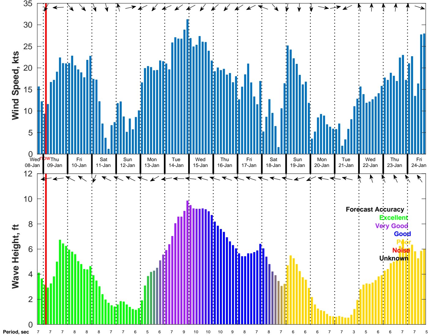
Wind & Wave Forecast for NDBC 42092 from 08-Jan-2025 18:00:00 to 24-Jan-2025 18:00:00
