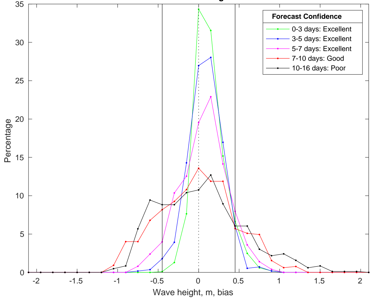
NDBC 44020 vs GFSWaves Bias Histogram: 09-Jan-2025
