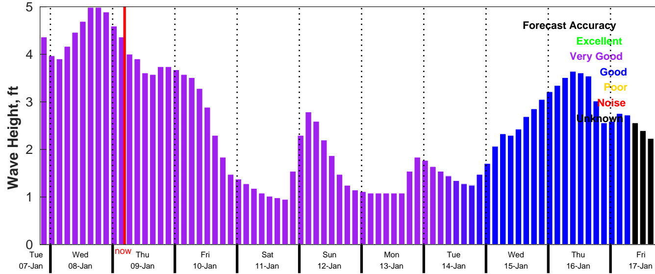
CMEMS Wave Forecast for NDBC 44020 from 07-Jan-2025 20:00:00 to 17-Jan-2025 20:00:00
