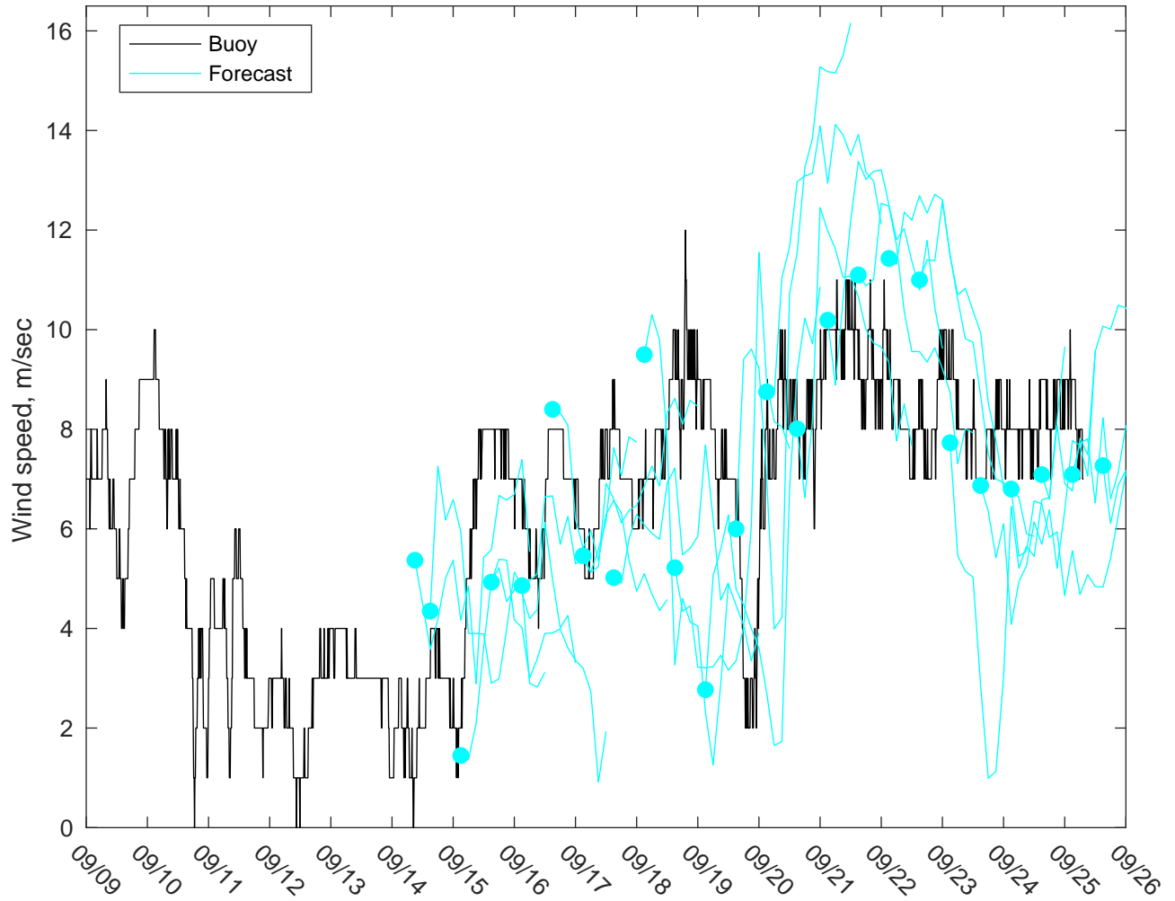
NDBC 44025 vs GFSWinds: 5 to 7 day forecast
