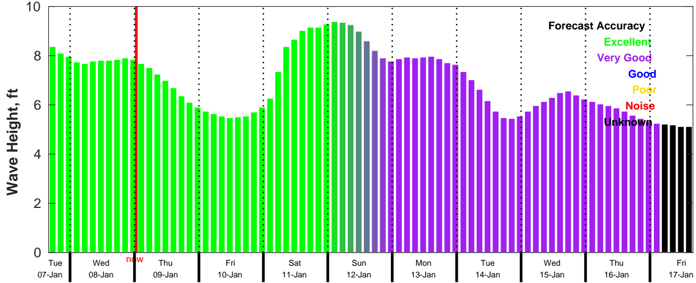
CMEMS Wave Forecast for NDBC 46011 from 07-Jan-2025 16:00:00 to 17-Jan-2025 16:00:00
