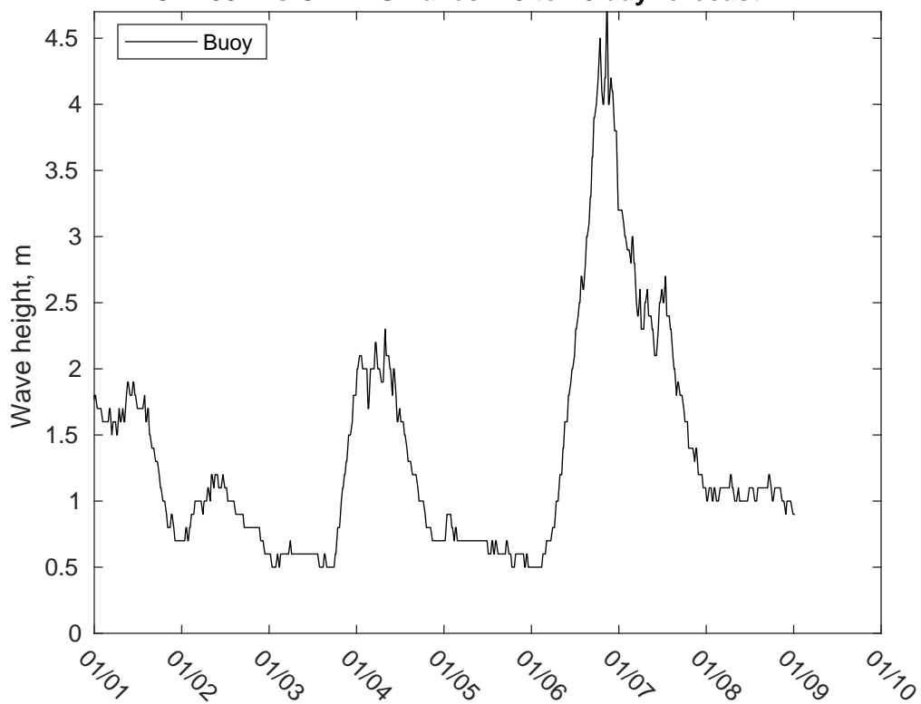
NDBC 41004 vs CMEMSWaves: 10 to 16 day forecast
