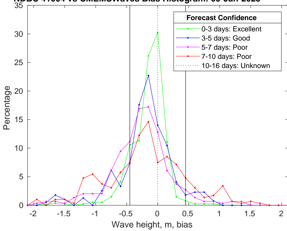
NDBC 41004 vs CMEMSWaves Bias Histogram: 09-Jan-2025
