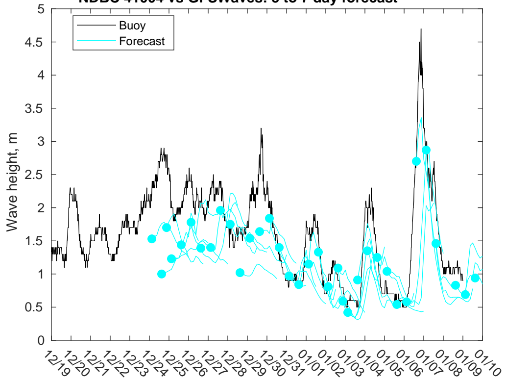
NDBC 41004 vs GFSWaves: 5 to 7 day forecast
