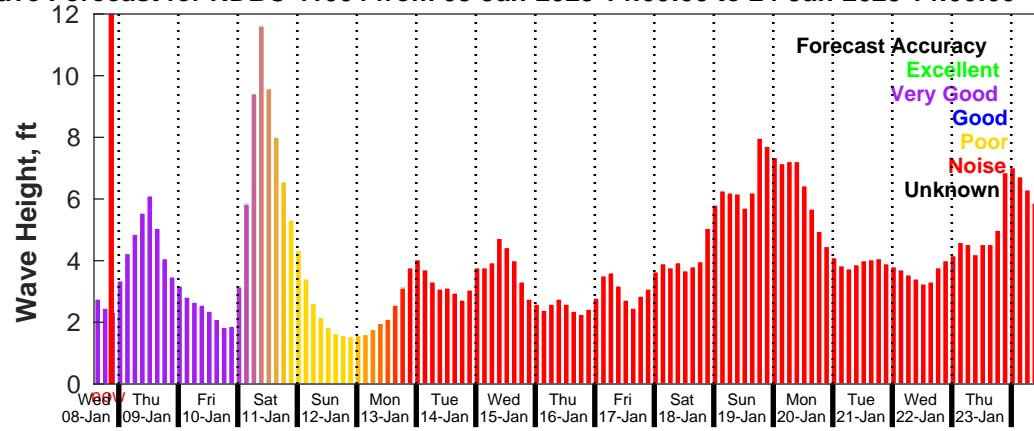
GFS Wave Forecast for NDBC 41004 from 08-Jan-2025 14:00:00 to 24-Jan-2025 14:00:00
