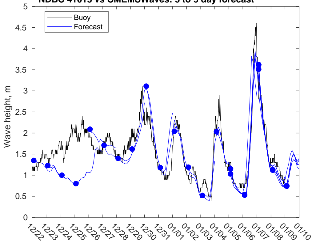
NDBC 41013 vs CMEMSWaves: 3 to 5 day forecast
