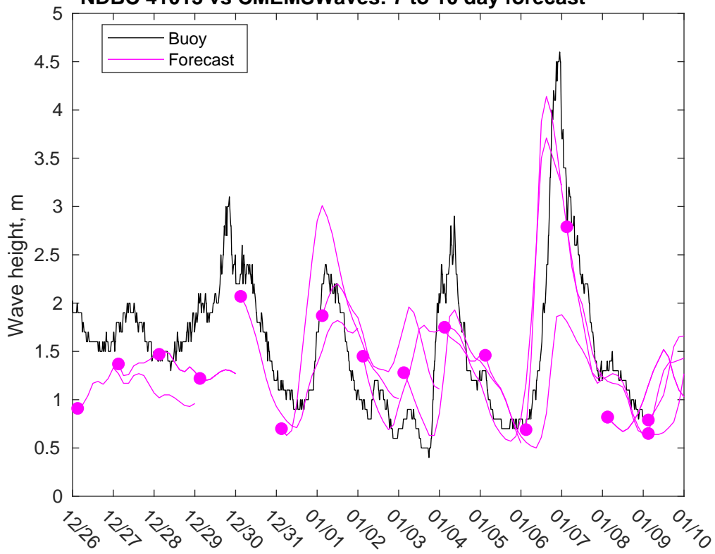
NDBC 41013 vs CMEMSWaves: 7 to 10 day forecast
