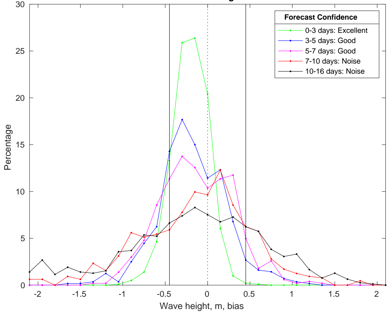
NDBC 42019 vs GFSWaves Bias Histogram: 09-Jan-2025
