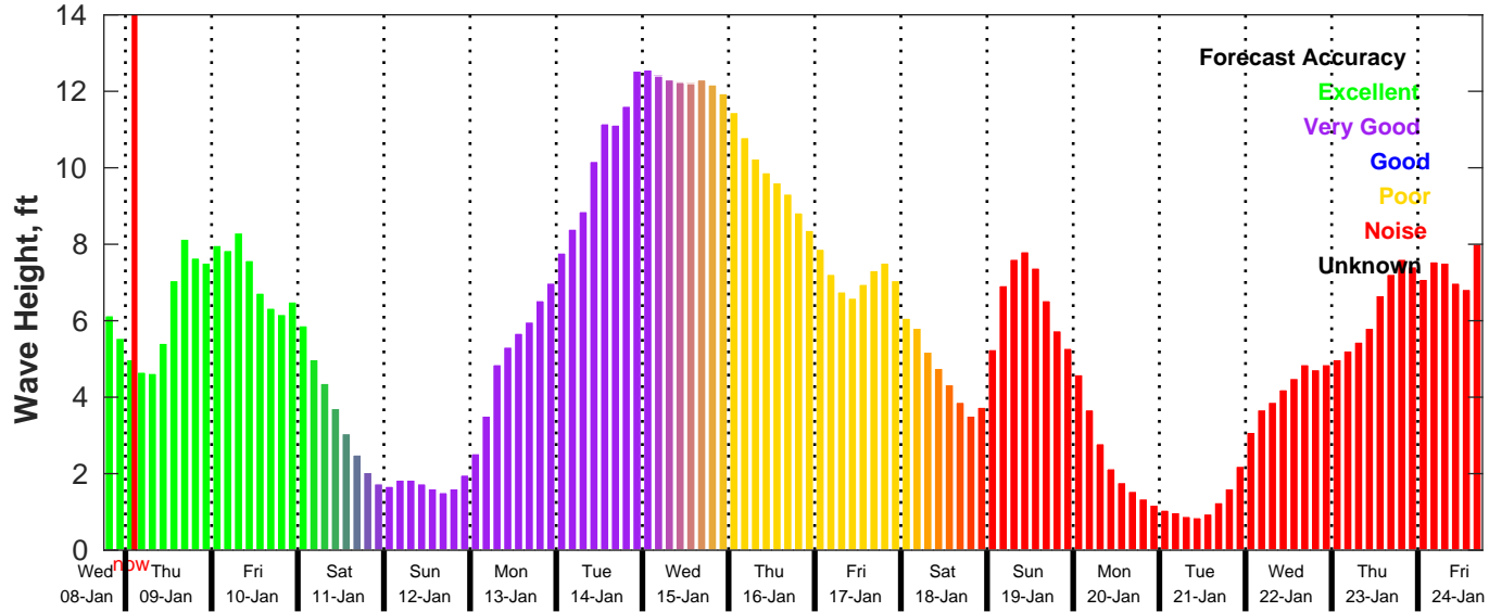
GFS Wave Forecast for NDBC 42020 from 08-Jan-2025 18:00:00 to 24-Jan-2025 18:00:00
