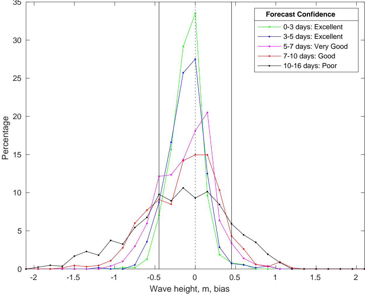
NDBC 42035 vs GFSWaves Bias Histogram: 09-Jan-2025
