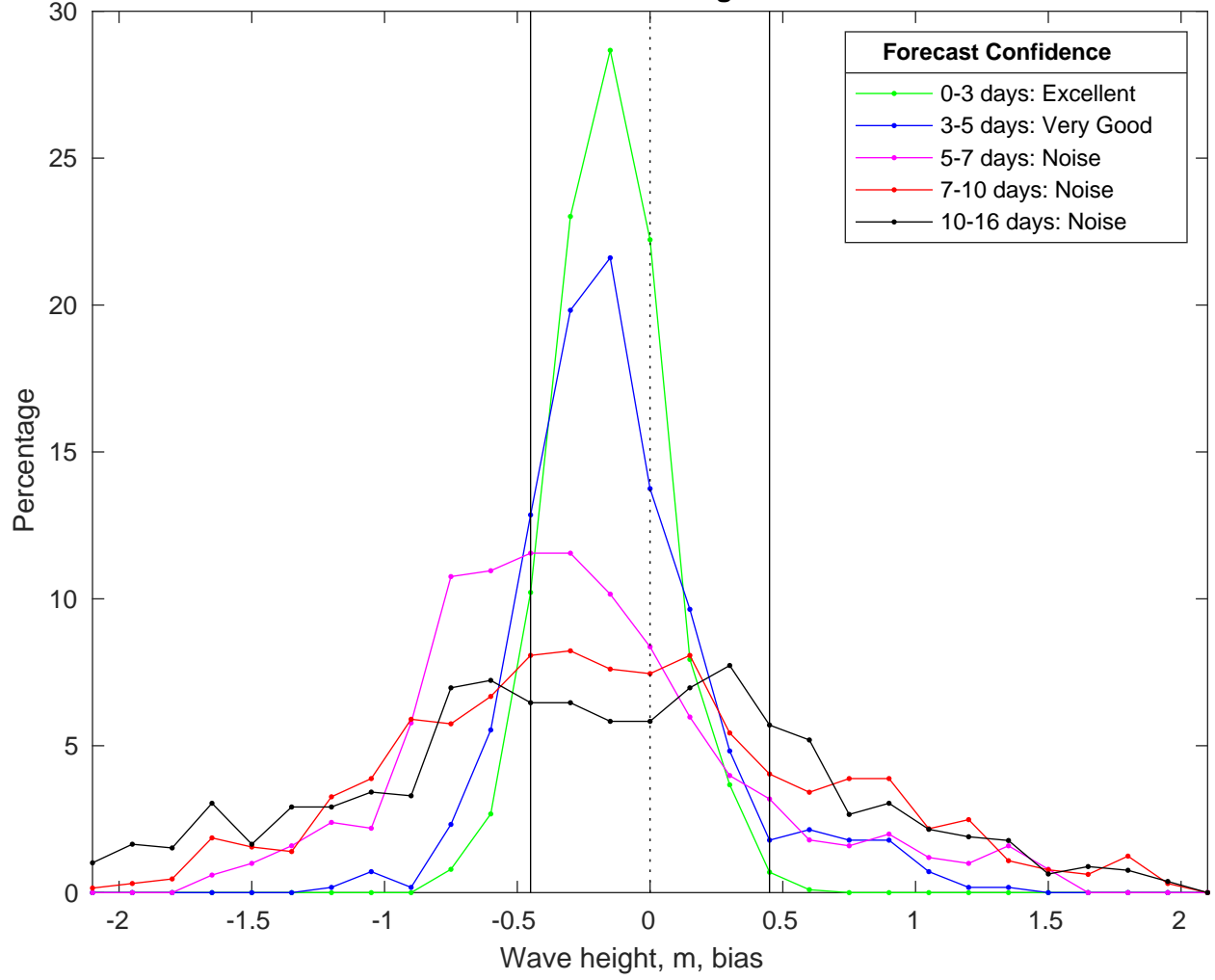
NDBC 42036 vs GFSWaves Bias Histogram: 09-Jan-2025
