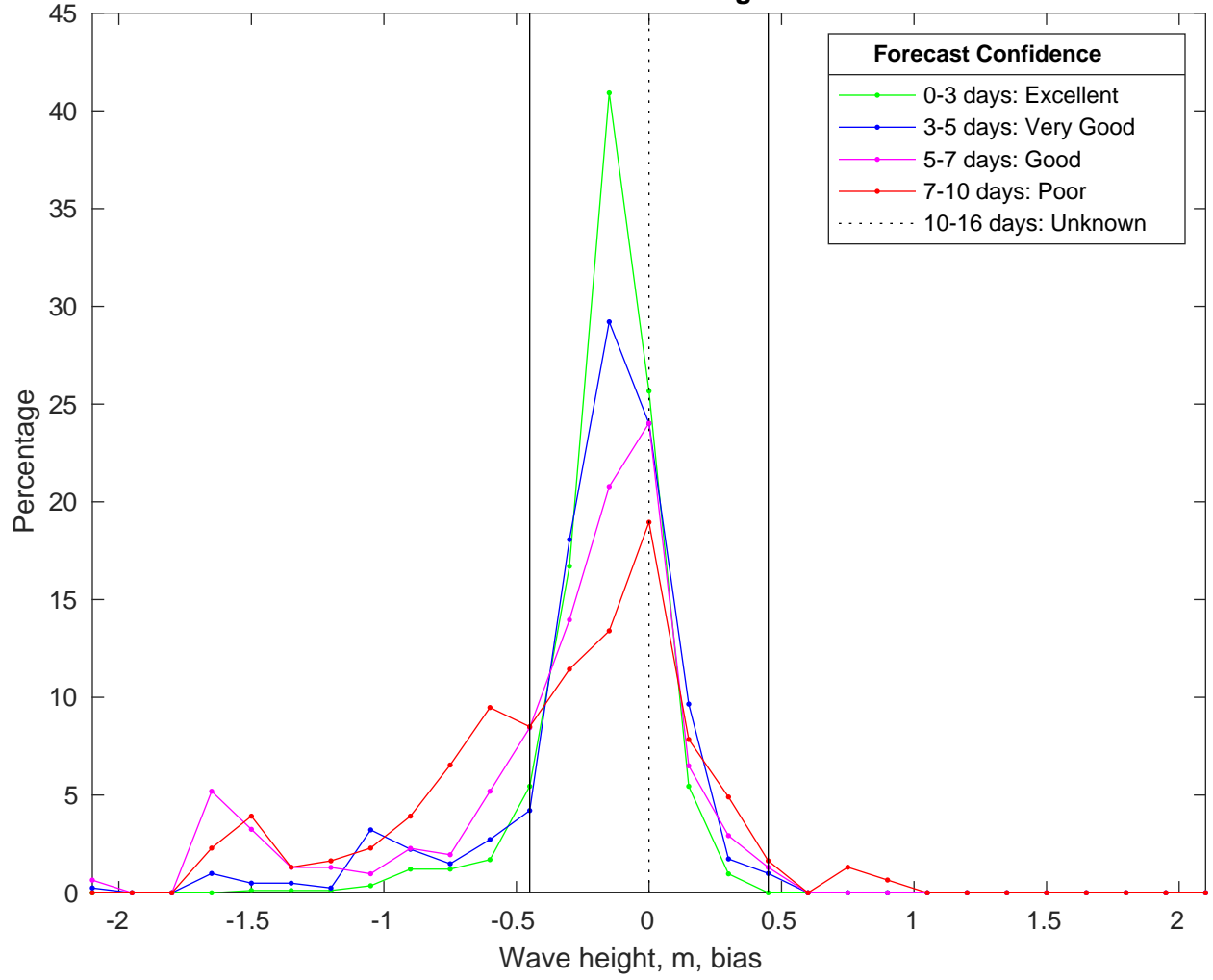
NDBC 42040 vs CMEMSWaves Bias Histogram: 09-Jan-2025
