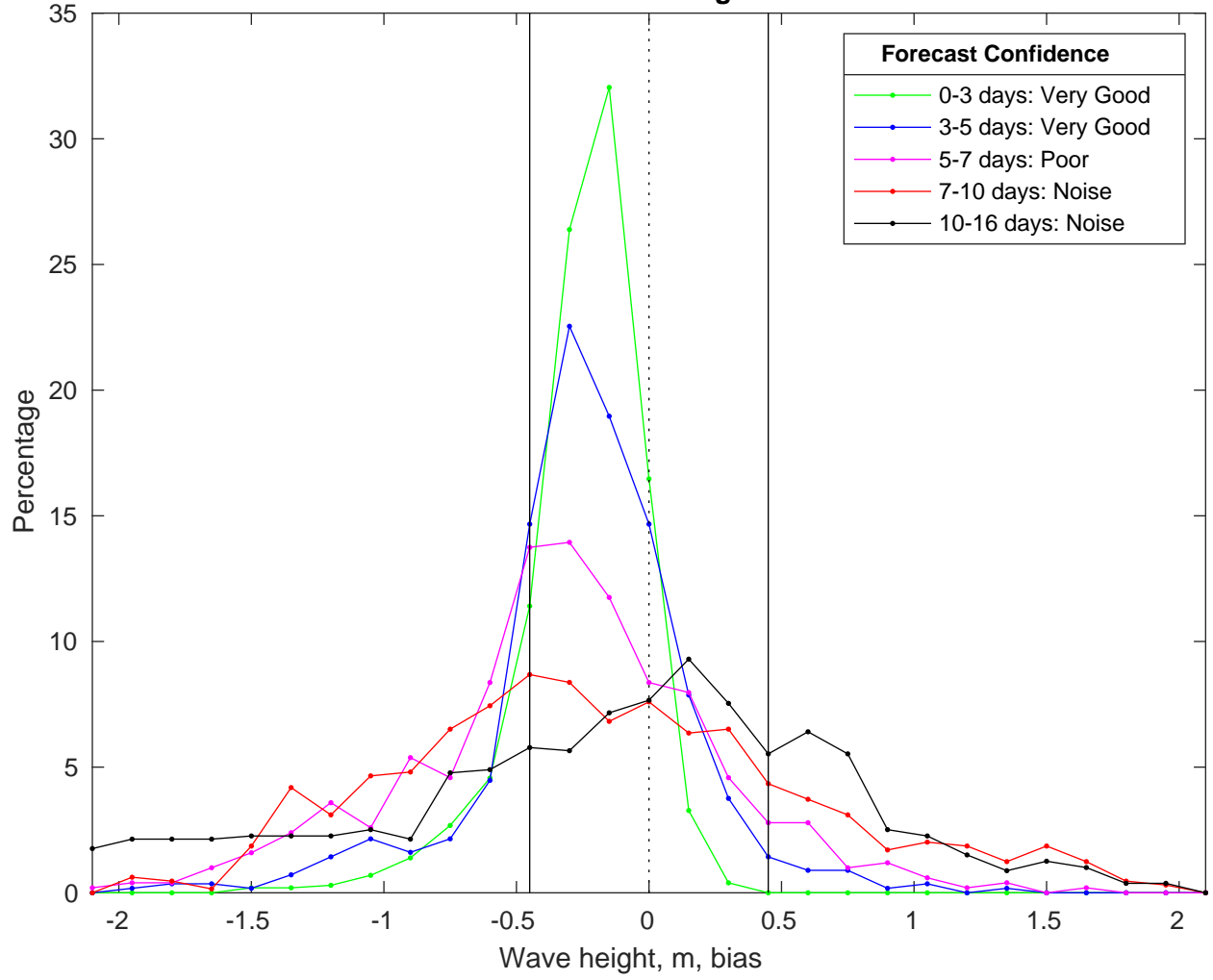
NDBC 42040 vs GFSWaves Bias Histogram: 09-Jan-2025
