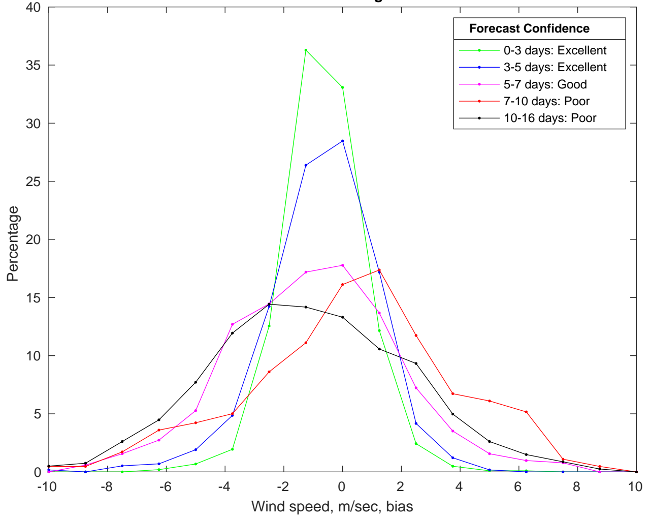
NDBC 42040 vs GFS Winds Bias Histogram: 26-Dec-2024
