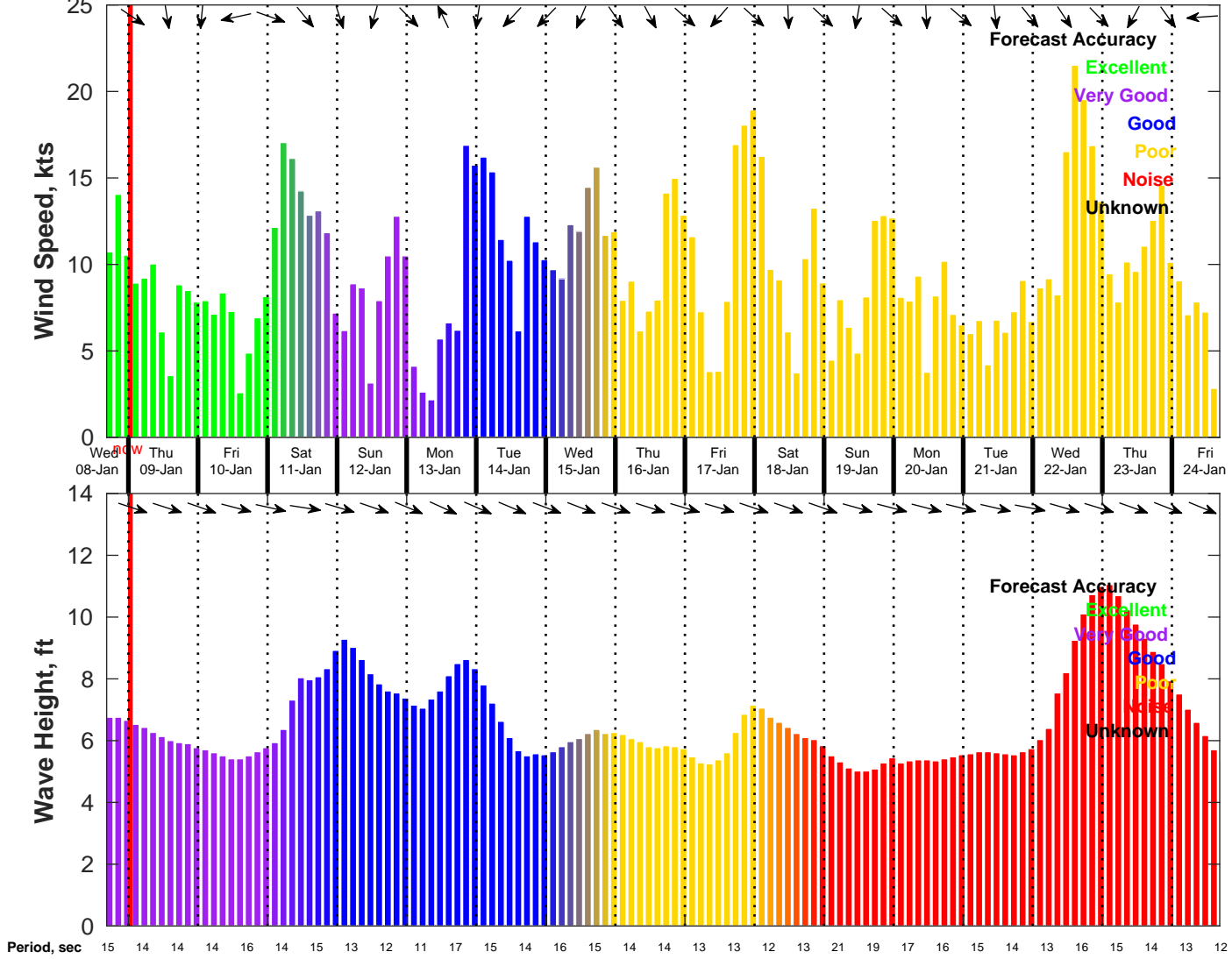
Wind & Wave Forecast for NDBC 46011 from 08-Jan-2025 16:00:00 to 24-Jan-2025 16:00:00
