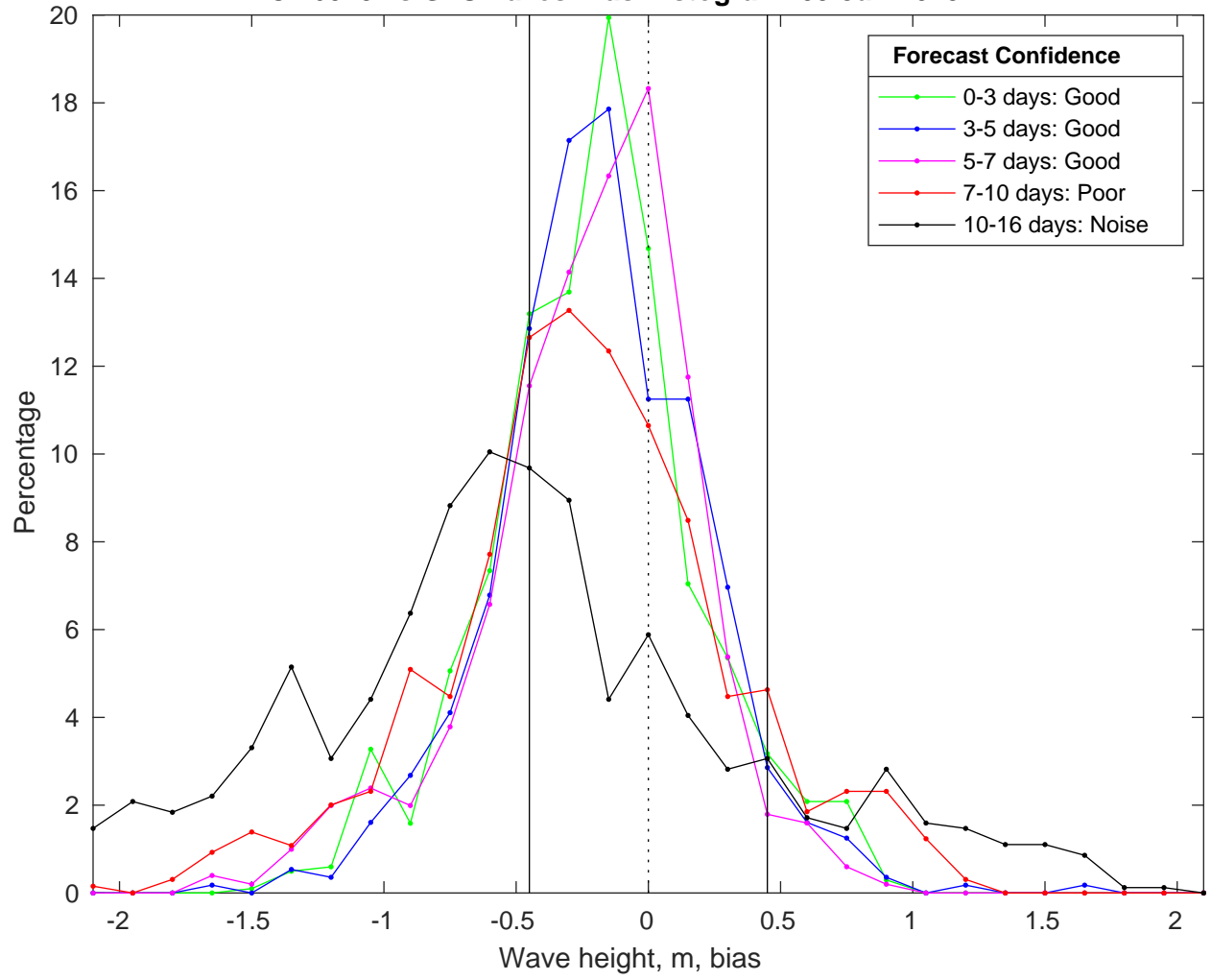
NDBC 46028 vs GFSWaves Bias Histogram: 09-Jan-2025
