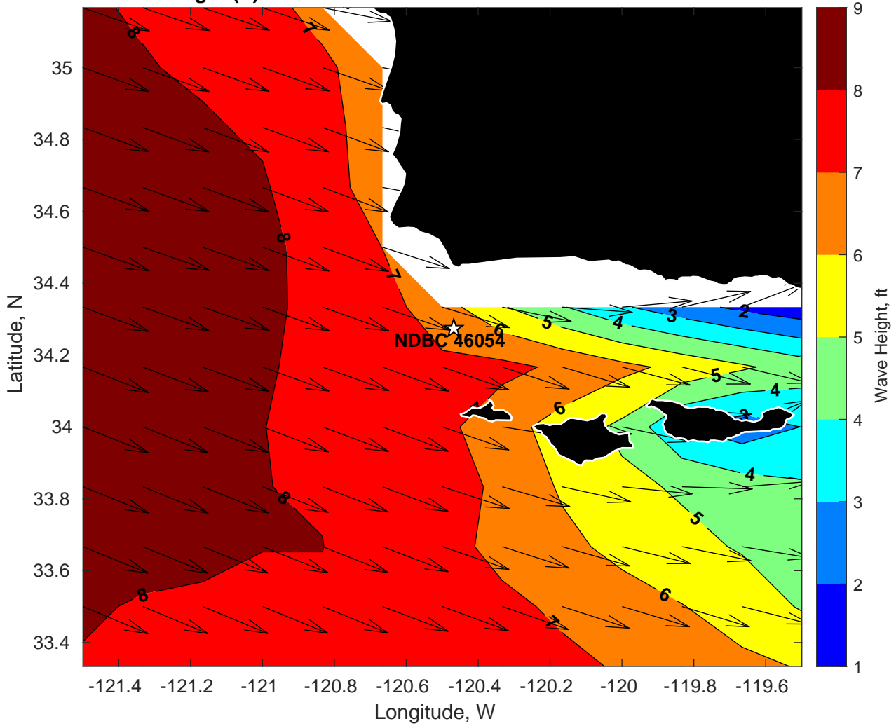
Wave Height (ft) for NDBC 46054 at 12-Dec-2024 21:00:00
