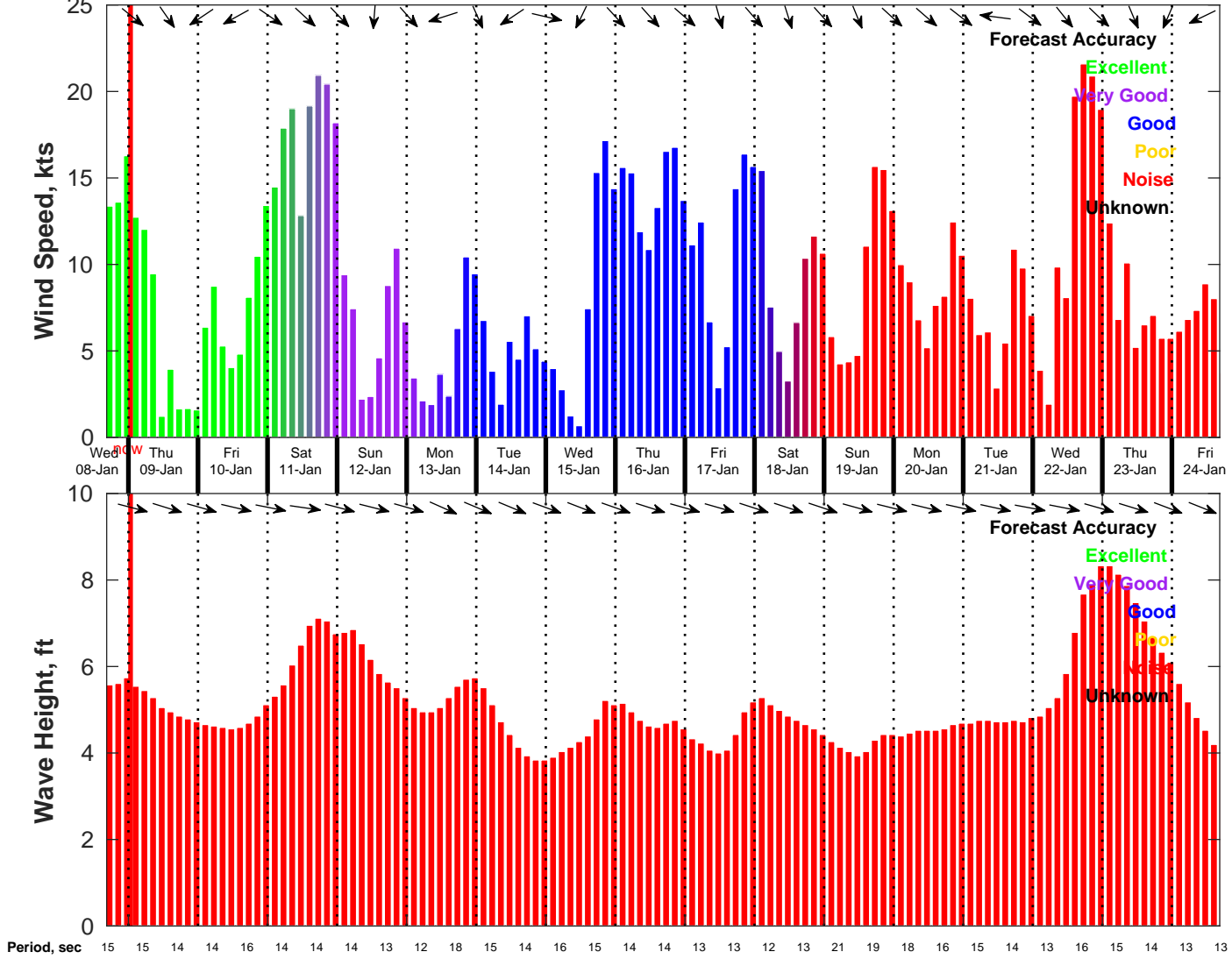
Wind & Wave Forecast for NDBC 46054 from 08-Jan-2025 16:00:00 to 24-Jan-2025 16:00:00
