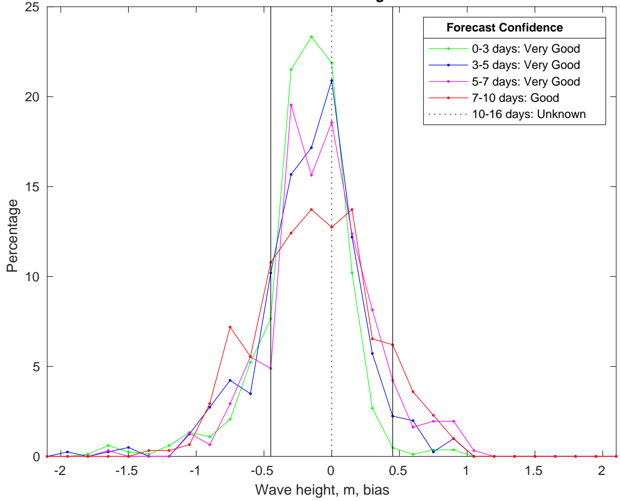
NDBC 46069 vs CMEMSWaves Bias Histogram: 09-Jan-2025
