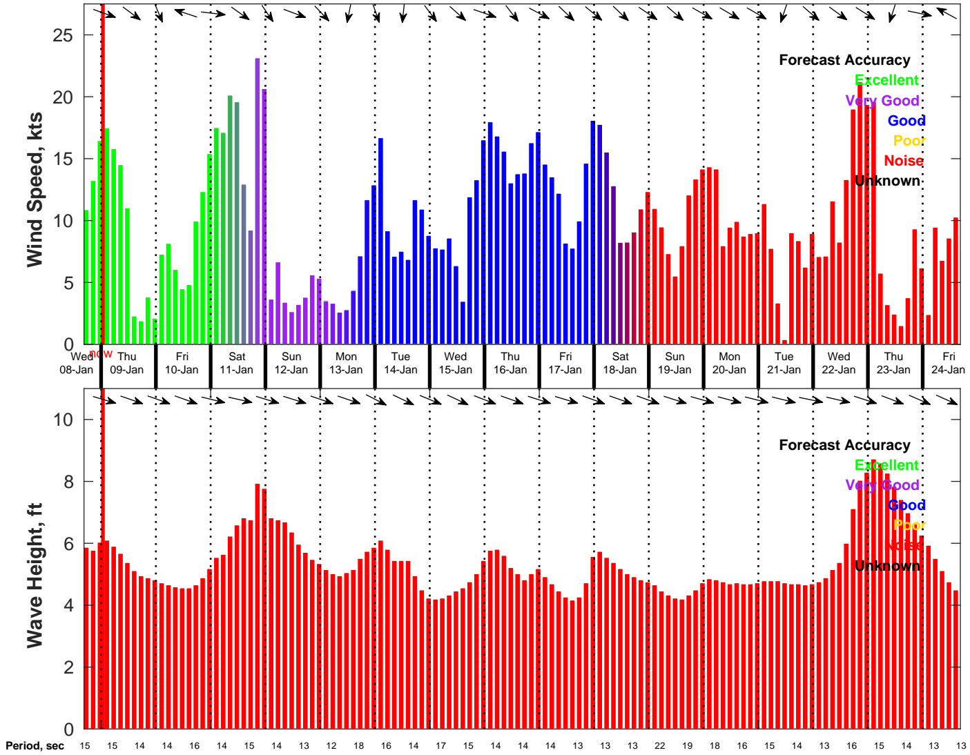
Wind & Wave Forecast for NDBC 46069 from 08-Jan-2025 16:00:00 to 24-Jan-2025 16:00:00
