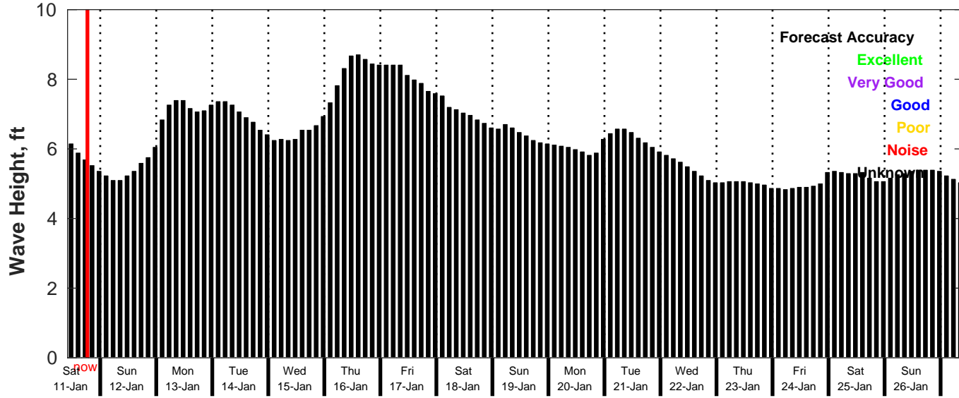
GFS Wave Forecast for NDBC 52211 from 10-Jan-2025 10:00:00 to 26-Jan-2025 10:00:00
