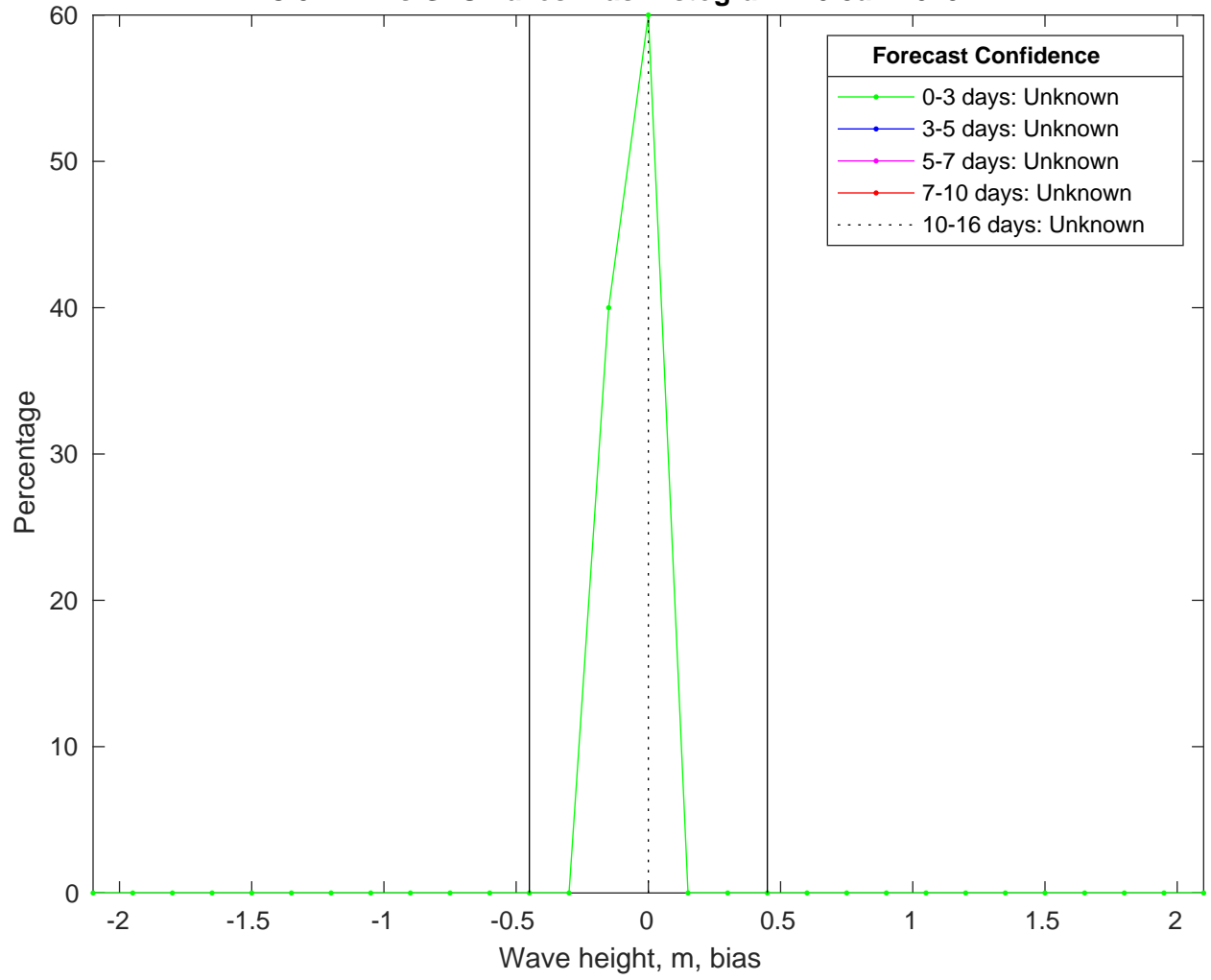
NDBC 52212 vs GFSWaves Bias Histogram: 10-Jan-2025
