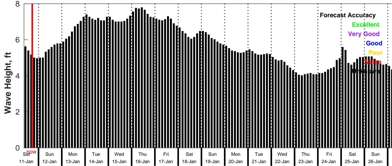
GFS Wave Forecast for NDBC 52212 from 10-Jan-2025 09:00:00 to 26-Jan-2025 09:00:00
