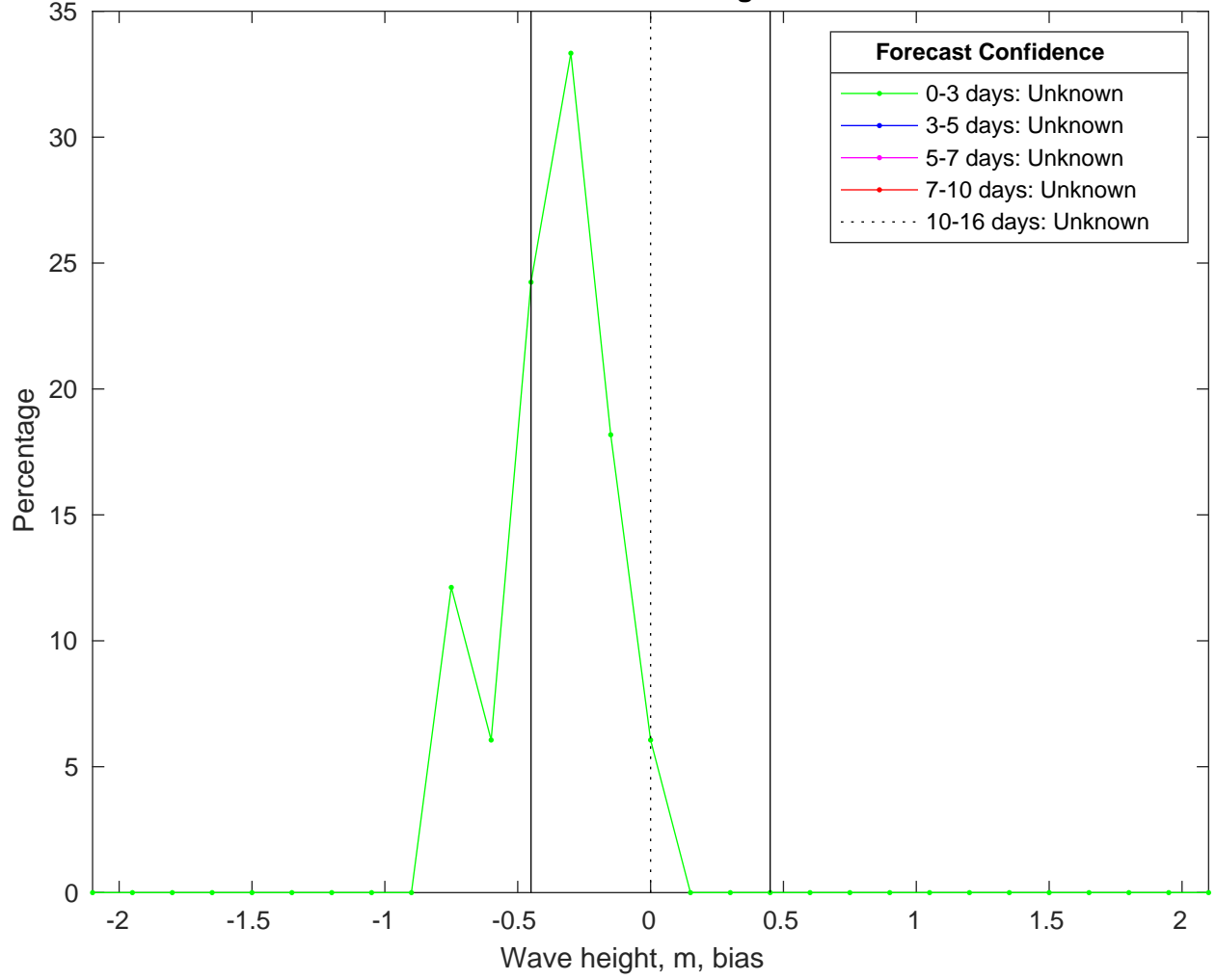
NDBC 52213 vs CMEMSWaves Bias Histogram: 10-Jan-2025
