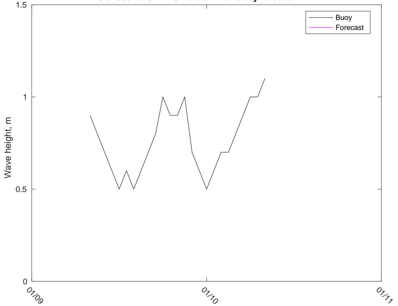
NDBC 62305 vs CMEMSWaves: 7 to 10 day forecast
