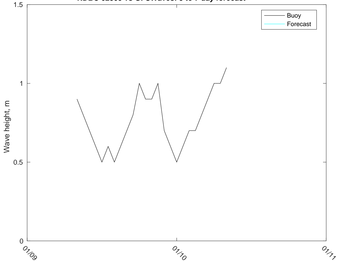
NDBC 62305 vs GFSWaves: 5 to 7 day forecast
