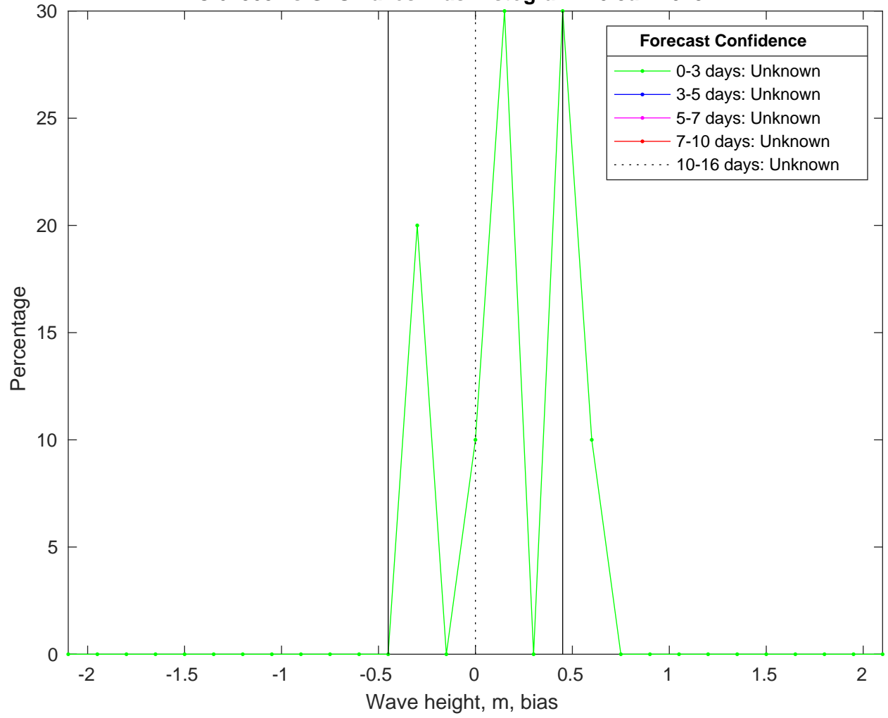
NDBC 62305 vs GFSWaves Bias Histogram: 10-Jan-2025
