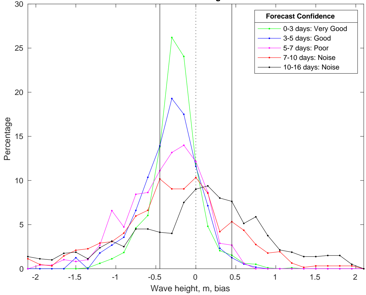
NDBC 41004 vs GFSWaves Bias Histogram: 11-Jan-2025
