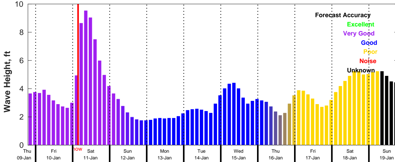
CMEMS Wave Forecast for NDBC 41004 from 09-Jan-2025 19:00:00 to 19-Jan-2025 19:00:00
