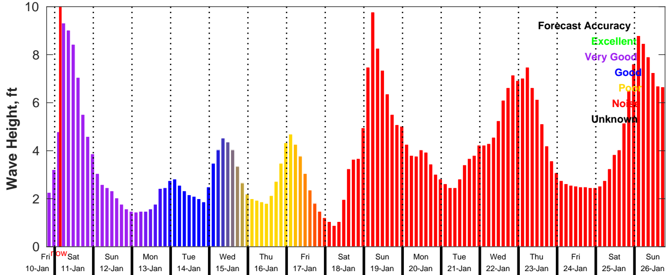
GFS Wave Forecast for NDBC 41004 from 10-Jan-2025 19:00:00 to 26-Jan-2025 19:00:00
