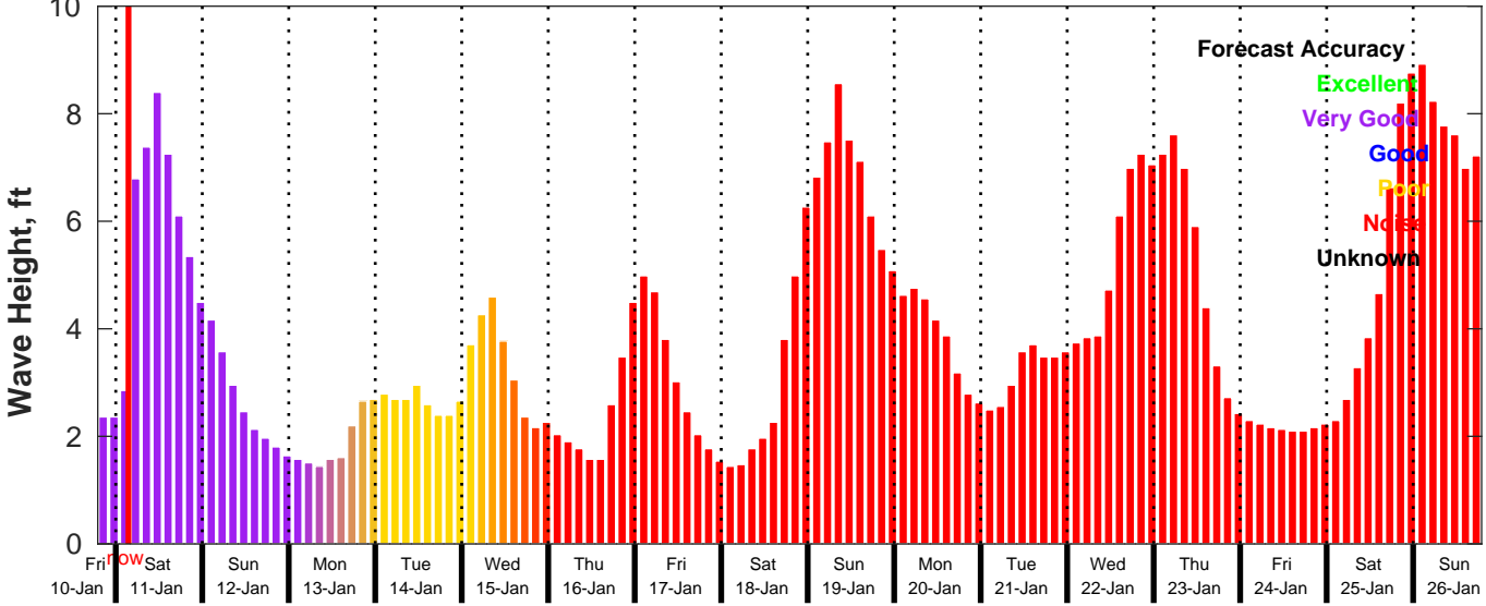
GFS Wave Forecast for NDBC 41013 from 10-Jan-2025 19:00:00 to 26-Jan-2025 19:00:00
