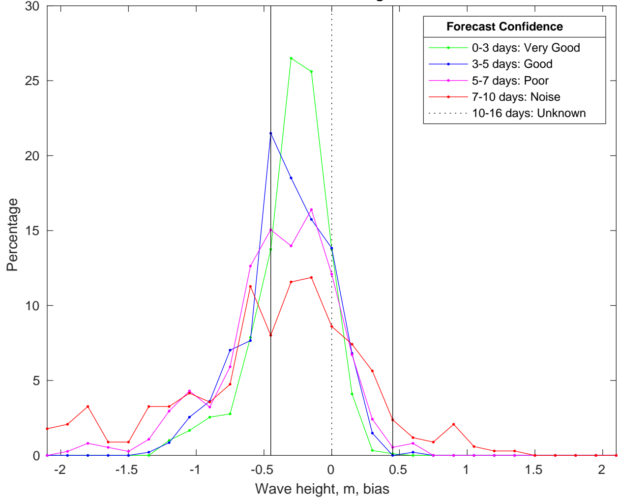
NDBC 42019 vs CMEMSWaves Bias Histogram: 11-Jan-2025
