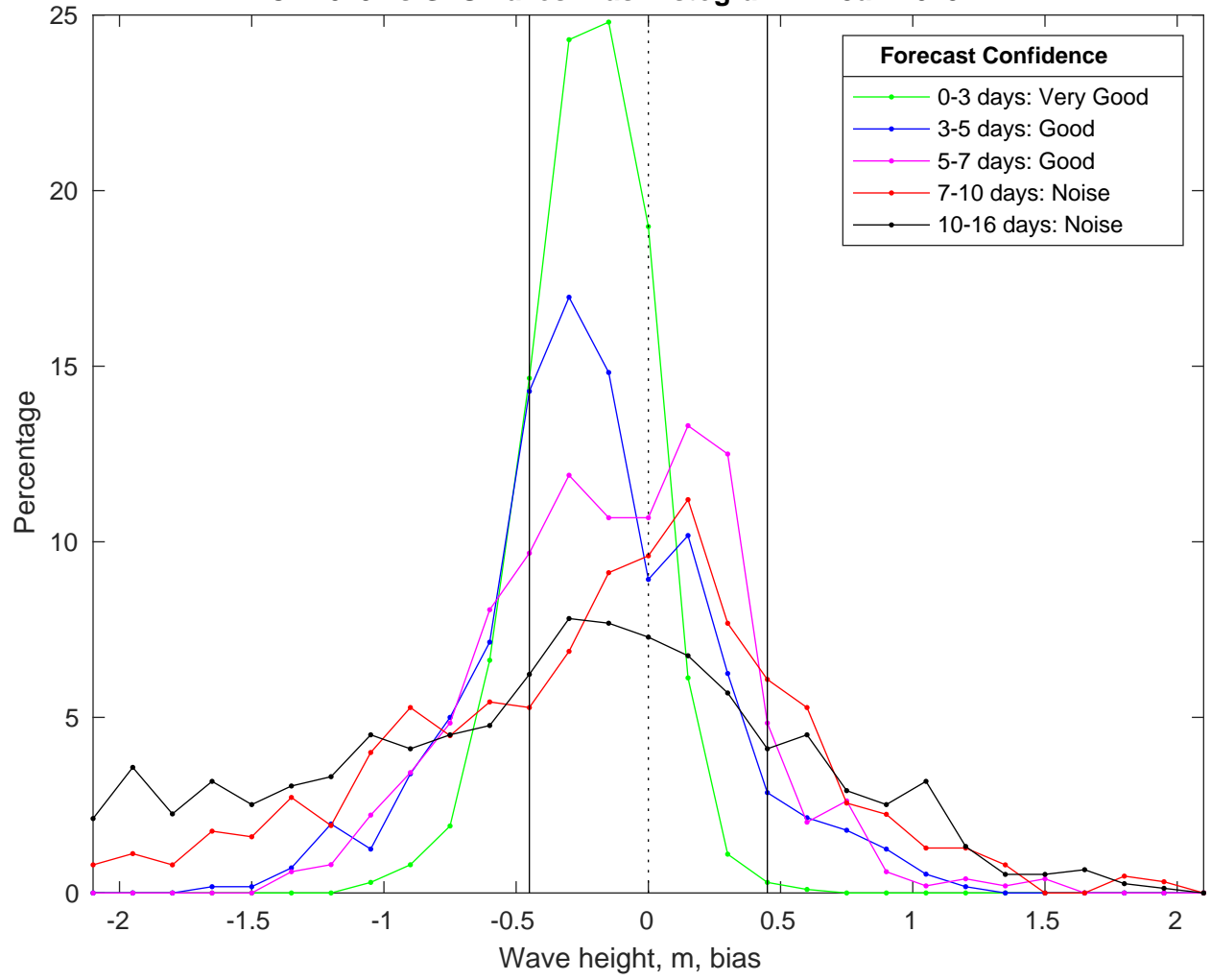
NDBC 42019 vs GFSWaves Bias Histogram: 11-Jan-2025
