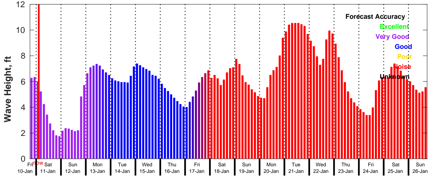
GFS Wave Forecast for NDBC 42019 from 10-Jan-2025 18:00:00 to 26-Jan-2025 18:00:00
