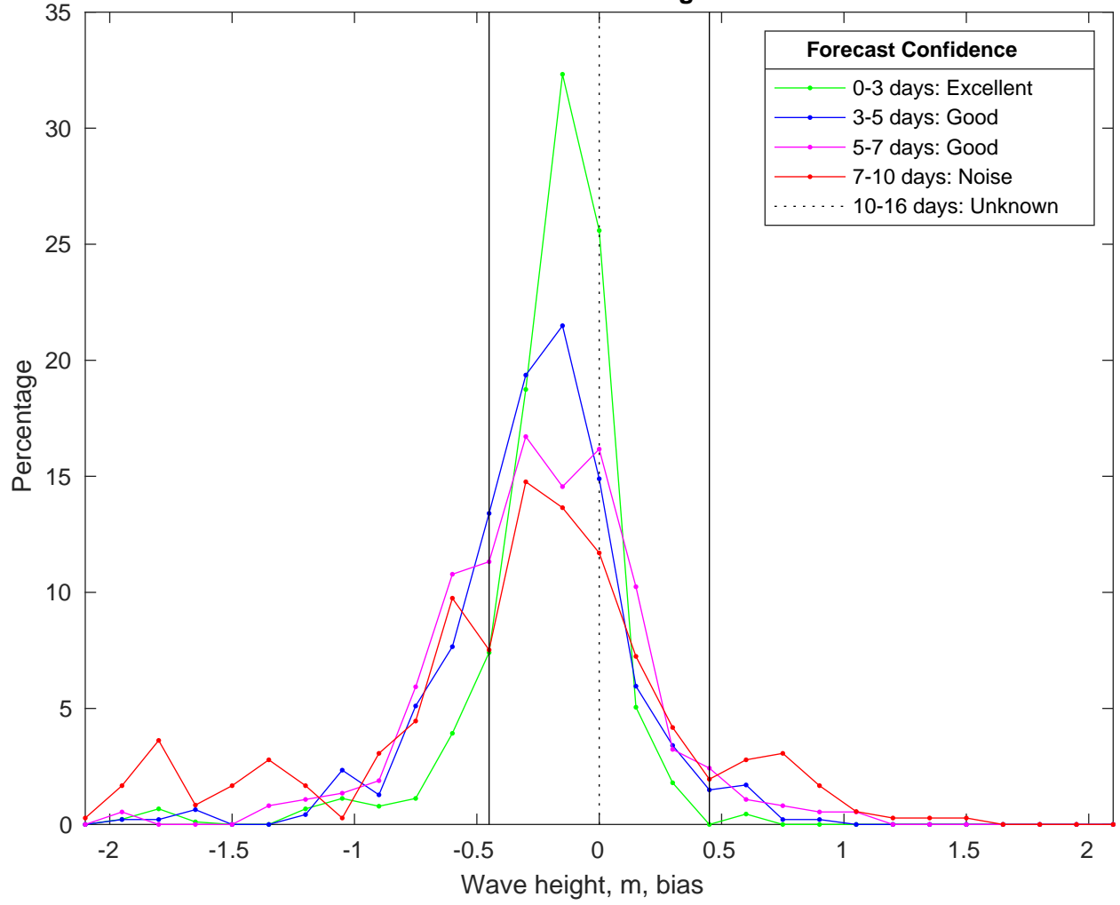
NDBC 42020 vs CMEMSWaves Bias Histogram: 11-Jan-2025
