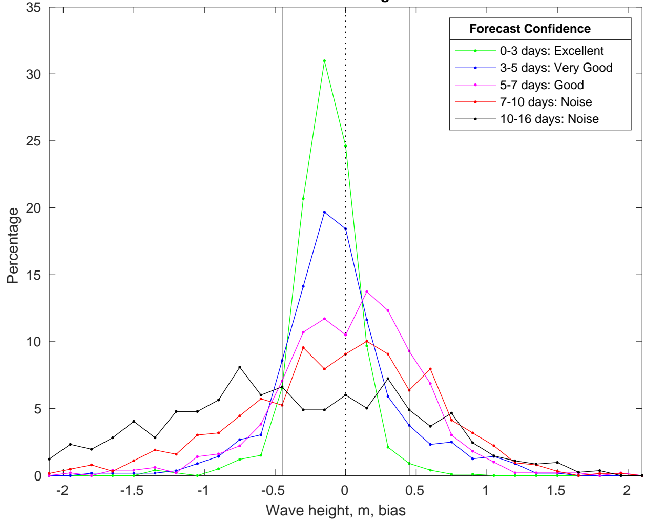
NDBC 42020 vs GFSWaves Bias Histogram: 11-Jan-2025
